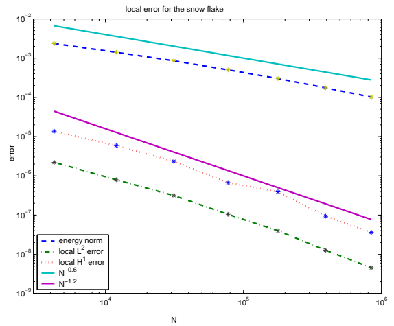
Figure 3: Domain and results corresponding to Example 3.2
