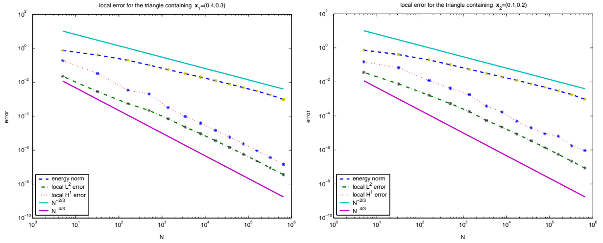
Figure 2: Results corresponding to Example 3.1
