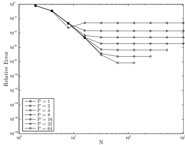
Figure 4.3: Relative error in the approximation (4.2) to the potential at the test point. Third example (Gaussian surface profile).
