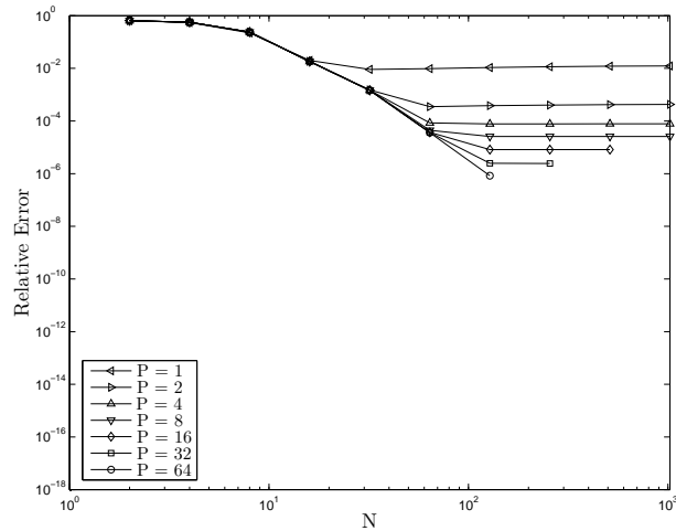
Figure 4.4: Relative \ell_2 error in normal velocity for the third example (Gaussian surface profile).
