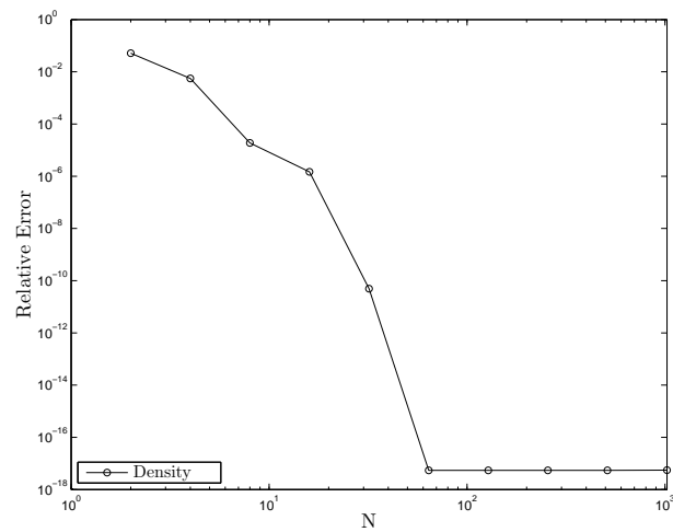
Figure 4.2: Relative \ell_2 error in density for the second example (flat surface)
