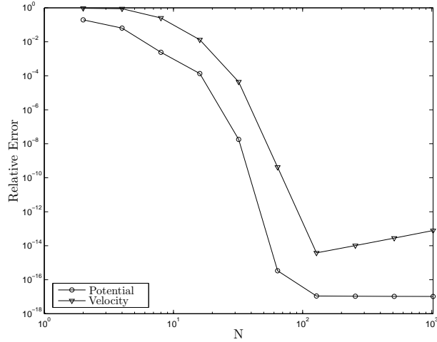
Figure 4.1: Relative errors in potential at the test point and in normal velocity for the first example (sinusoidal surface profile).
